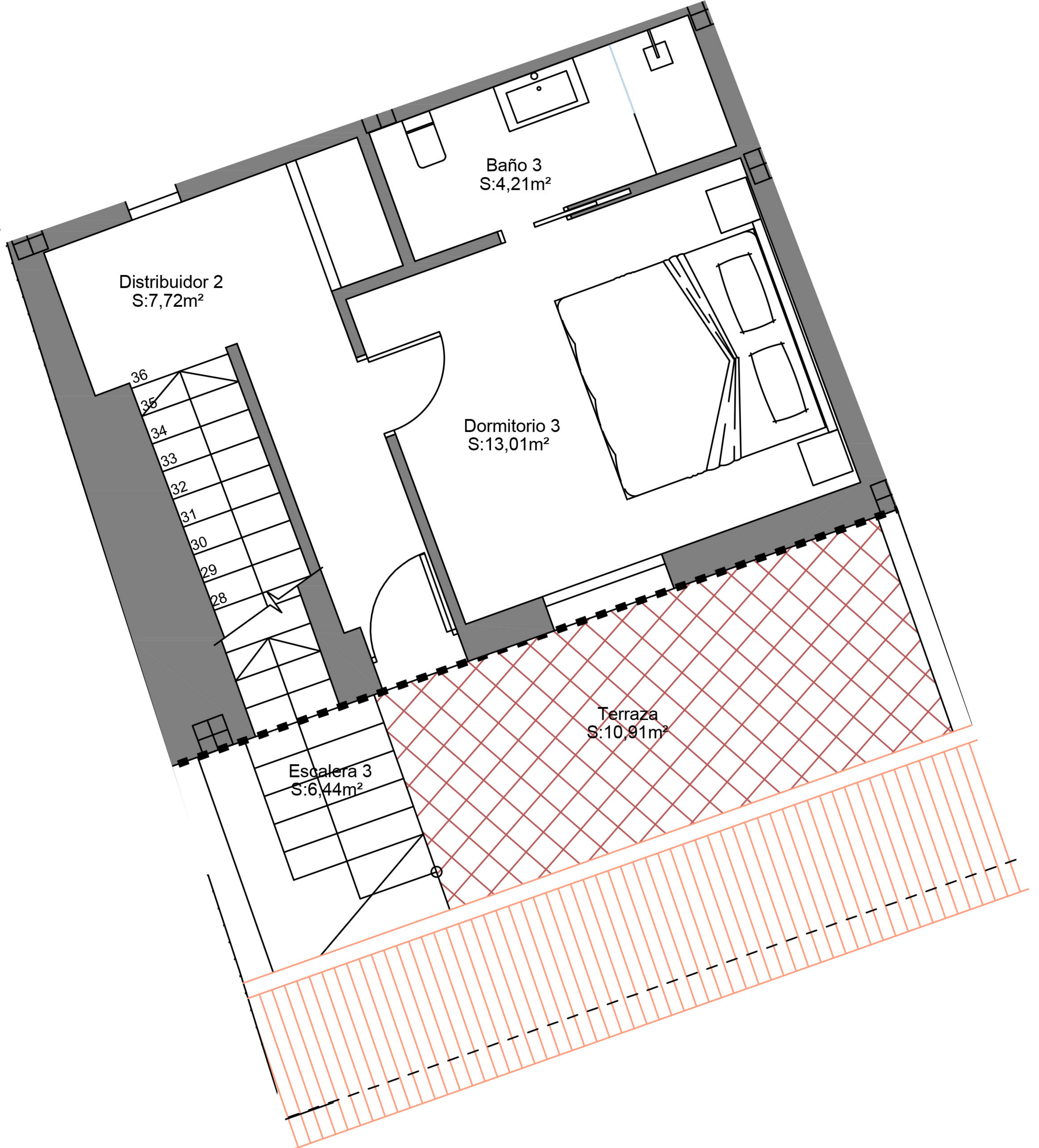
TOP FLOOR
