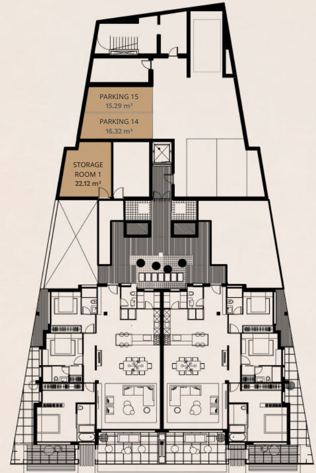
FLOOR -2
