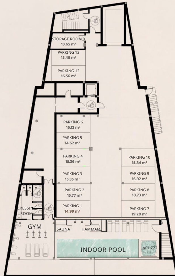
FLOOR -3
