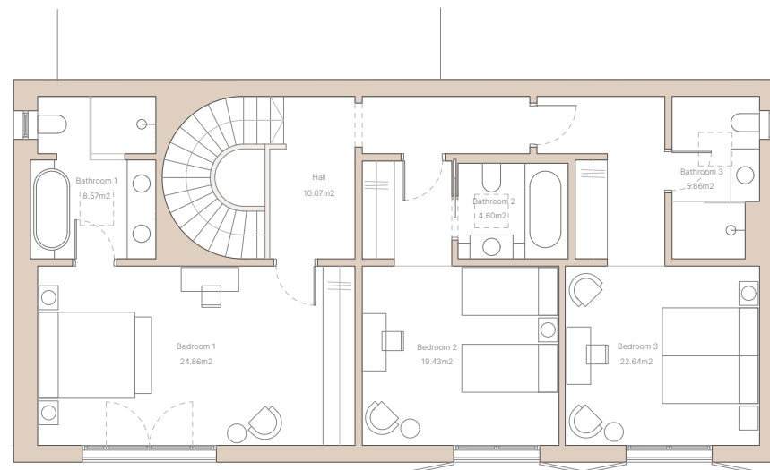
PLANTA ALTA FIRST FLOOR
