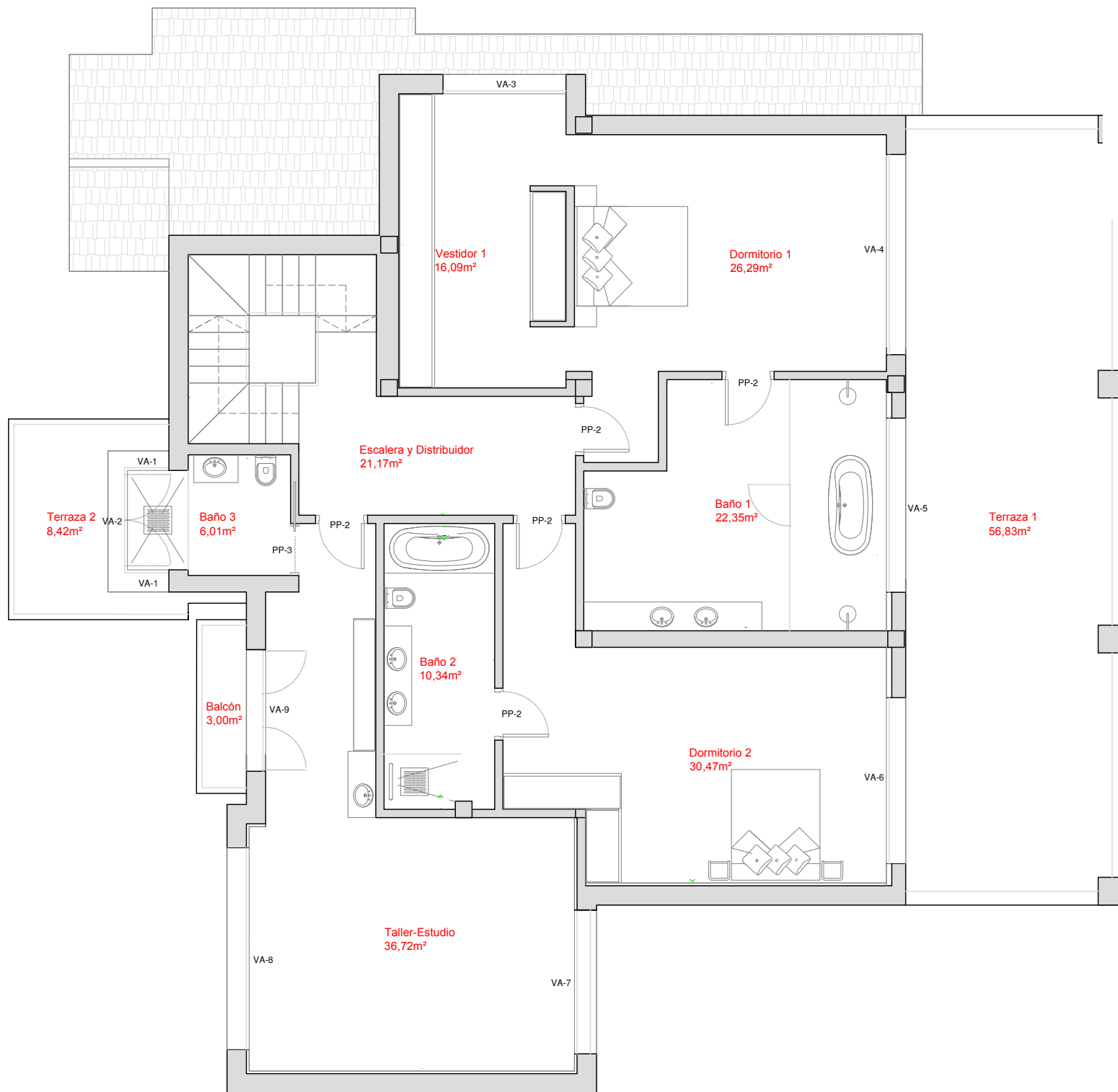
PLANTA ALTA / FIRST FLOOR
